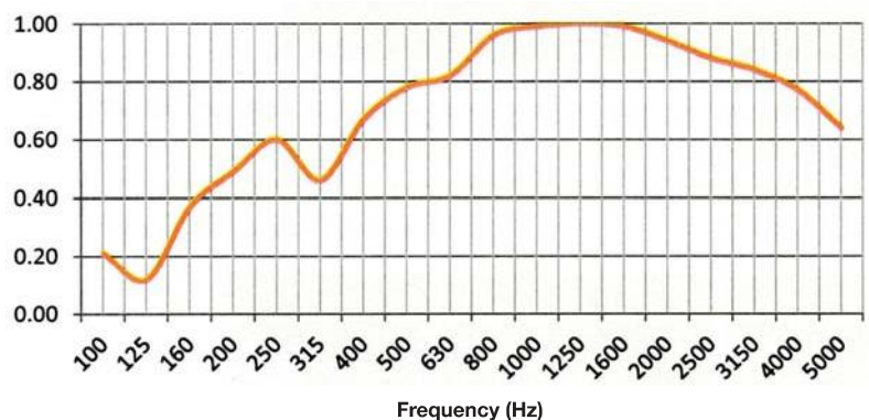
Absorption coefficient (polyester fiber)
